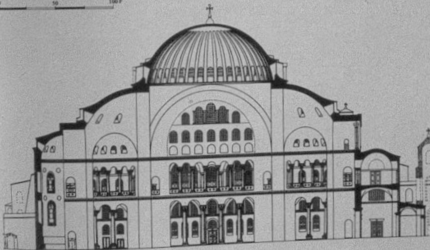
94. Constantinople, St Sophia. Cross-Section (east-west axis). 95. Constantinople, St Sophia. Cross-Section (north-south axis).
